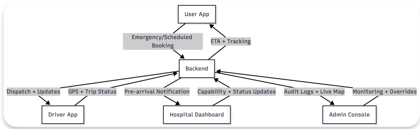
System Overview Flow
