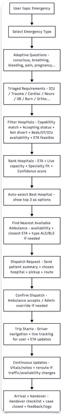
Emergency Booking & Dispatch Flow
