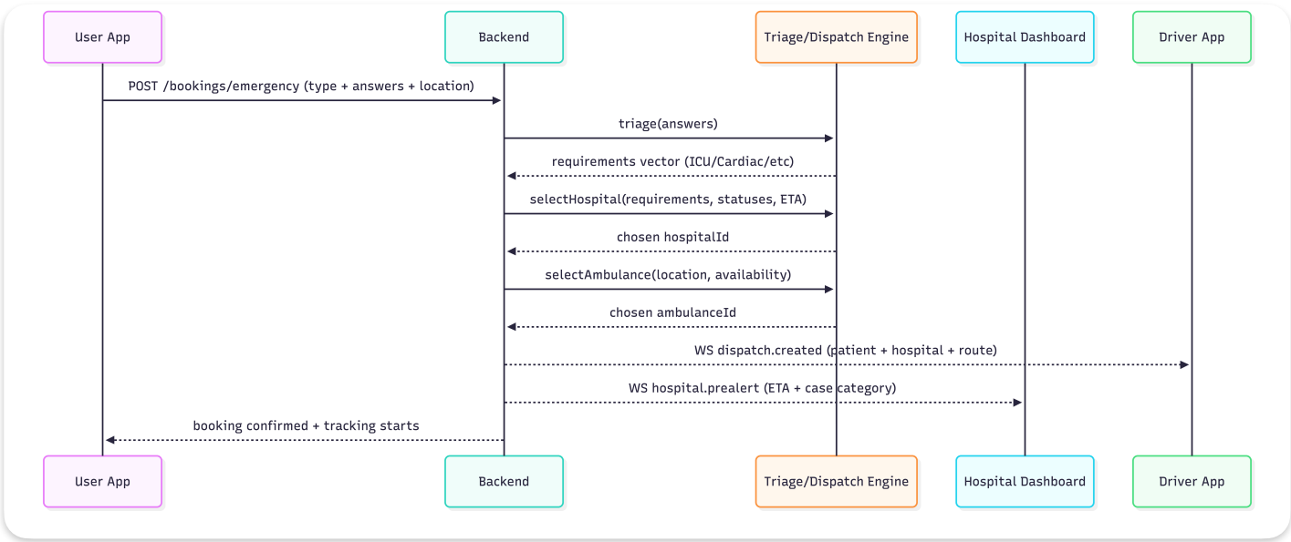
Emergency Dispatch Sequence Diagram
