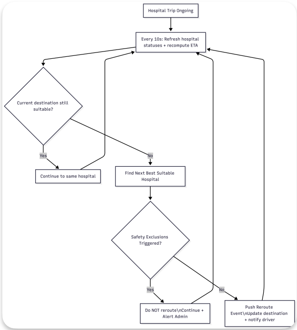
Real-time Re-routing Flow (with Safety Exclusions)
